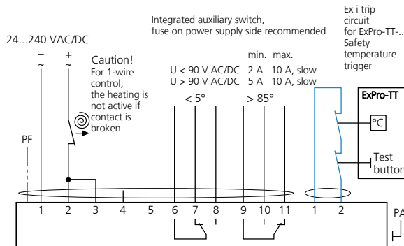
Fig. 22: SB7.2 - cable type 10+PE, cable diameter 9.4 mm
