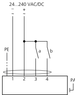
Fig. 3: SB1.0 - cable type 4+PE, cable diameter 7.2 mm
