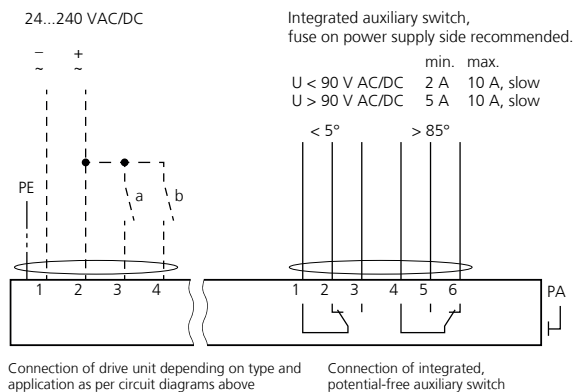
Fig. 10: SB3.0 - cable type 5+PE, cable diameter 7.5 mm / cable type 6, cable diameter 7.4 mm
