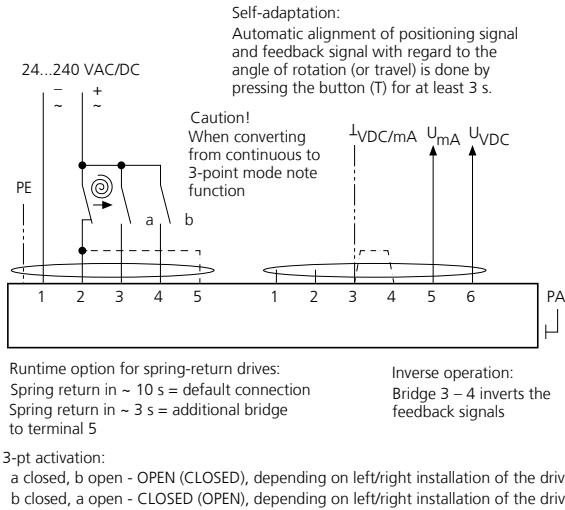
Fig. 17: SB5.3 - cable type 5+PE, cable diameter 7.5 mm / cable type 6, cable diameter 7.4 mm
