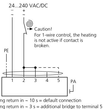
Fig. 5: SB2.1 - cable type 5+PE, cable diameter 7.5 mm
