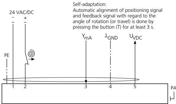
Fig. 19: SB6.1 - cable type 5+PE, cable diameter 7.5 mm
