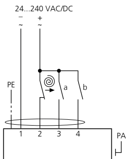
Fig. 6: SB2.2 - cable type 4+PE, cable diameter 7.2 mm
