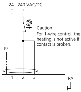
Fig. 9: SB2.5 - cable type 3+PE, cable diameter 6 mm
