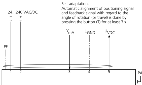
Fig. 18: SB6.0 - cable type 5+PE, cable diameter 7.5 mm
