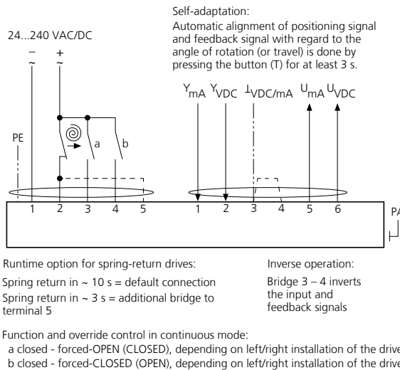
Fig. 14: SB5.0 - cable type 5+PE, cable diameter 7.5 mm / cable type 6, cable diameter 7.4 mm
