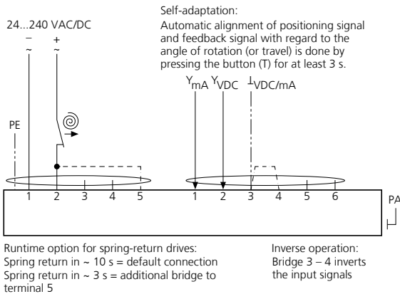
Fig. 16: SB5.2 - cable type 5+PE, cable diameter 7.5 mm / cable type 6, cable diameter 7.4 mm
