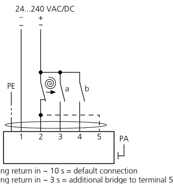
Fig. 4: SB2.0 - cable type 5+PE, cable diameter 7.5 mm
