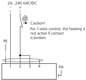
Fig. 7: SB2.3 - cable type 4+PE, cable diameter 7.2 mm
