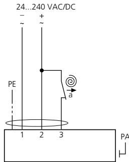
Fig. 8: SB2.4 - cable type 3+PE, cable diameter 6 mm
