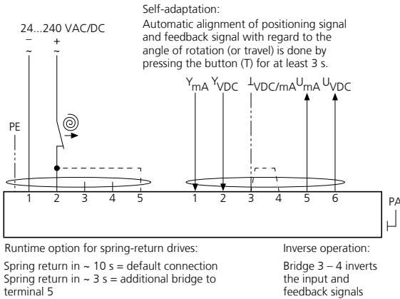
Fig. 15: SB5.1 - cable type 5+PE, cable diameter 7.5 mm / cable type 6, cable diameter 7.4 mm
