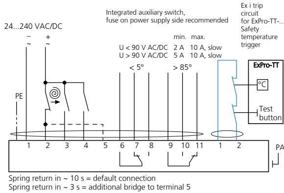
Fig. 21: SB7.1 - cable type 11+PE, cable diameter 9.9 mm
