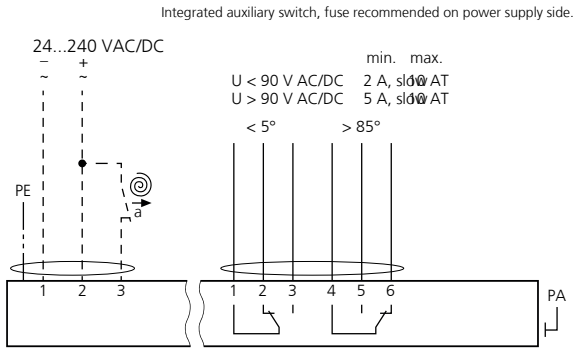
Fig. 11: SB3.2 - Connection of the integrated potential-free auxiliary switch
