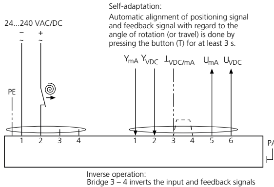
Fig. 13: SB4.1 - cable type 4+PE, cable diameter 7.2 mm / cable type 6, cable diameter 7.4 mm
