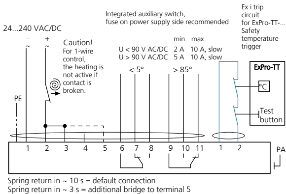
Fig. 20: SB7.0 - cable type 11+PE, cable diameter 9.9 mm
